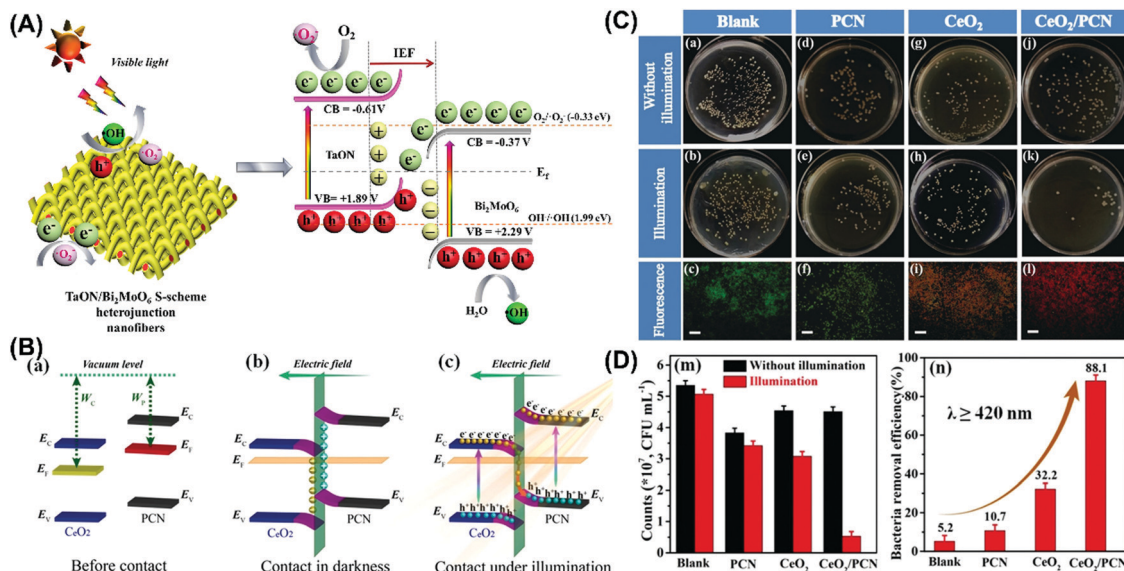
Fig. 22 Photogenerated electron transfer and photocatalytic inactivation of S-scheme heterojunctions. (A) Photogenerated electron transport mechanism of S-scheme heterostructure (TaON/Bi 2 MoO 6 as an example). (B) Electron transfer and photocatalytic inactivation effects and numerical calculation of CeO 2 /PCN with different conditions. (A) Reprinted from ref. 297. (B)–(D) Reprinted from ref. 298.
