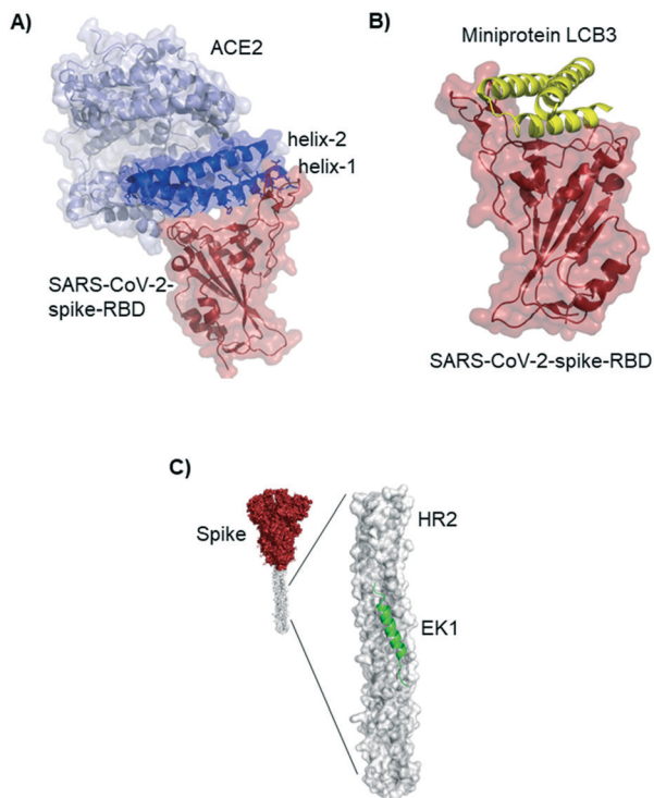
Fig. 3 ACE2 derived and de novo designed miniproteins and peptides binding to the SARS-CoV-2-spike protein. A) Crystal structure (6m0j) of ACE2 (blue) bound to SARS-CoV-2-spike-RBD (red). The ACE2 N-terminal helix-1 contains most of the residues interacting with the RBD and has been used as starting point for several design strategies for SARS-CoV-2 inhibitors. B) Cryo-EM structure (7jzm) of a computationally designed miniprotein (yellow cartoon) neutralizing SARS-CoV-2 in picomolar concentrations. C) Structural model (5zuv) of the fusion inhibitor EK1 (green cartoon) bound to the heptad repeat domain of the SARS-CoV-2 (grey surface).
