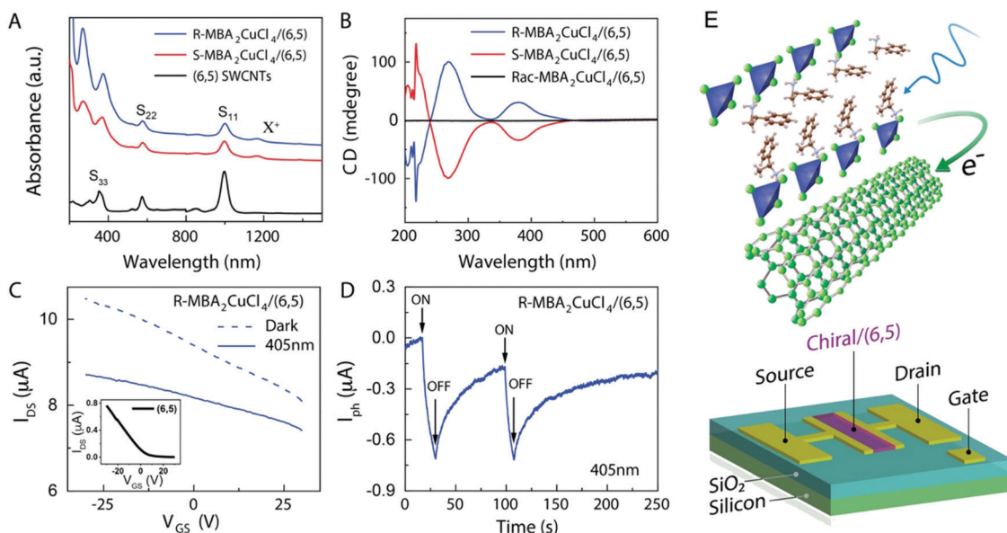
Fig. 13 (A) UV-Vis-NIR absorption spectra of SWCNT, R - and S - MBA_2CuCl_4/SWCNT . (B) CD signals of R - and S - MBA_2CuCl_4/(6,5) SWCNT and (rac-MBA)_2CuCl_4/(6,5) SWCNT. (C) A comparison of the effects of dark and photoresponse conditions on the FET transfer curve. (D) The photocurrent response of (R-MBA)_2CuCl_4/SWCNT over time. (E) A schematic description of a three-terminal FET device. Reprinted with permission. 104 Copyright 2021, American Chemical Society.
