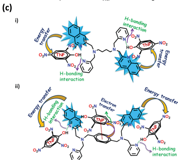
Fig. 6 (a) Schematic illustration of the quenching mechanism via photo-induced electron transfer. (b) Calculated energy diagram with the HOMO–LUMO energies of 1 , 2 and TNP. (c) Possible mechanism of TNP sensing in (i) 1 and (ii) 2 .
