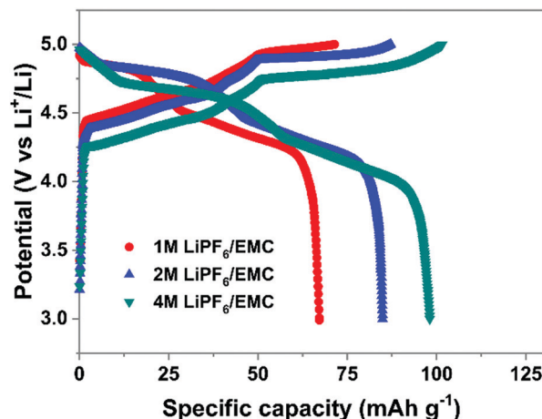
Fig. 11 Charge-discharge profiles of the graphite cathode in different concentration electrolytes. Li//graphite half cells were used. Electrolytes are 1–4 M \text{LiPF}_6 in EMC. The current density is 100 mA \text{g}^{-1} .
