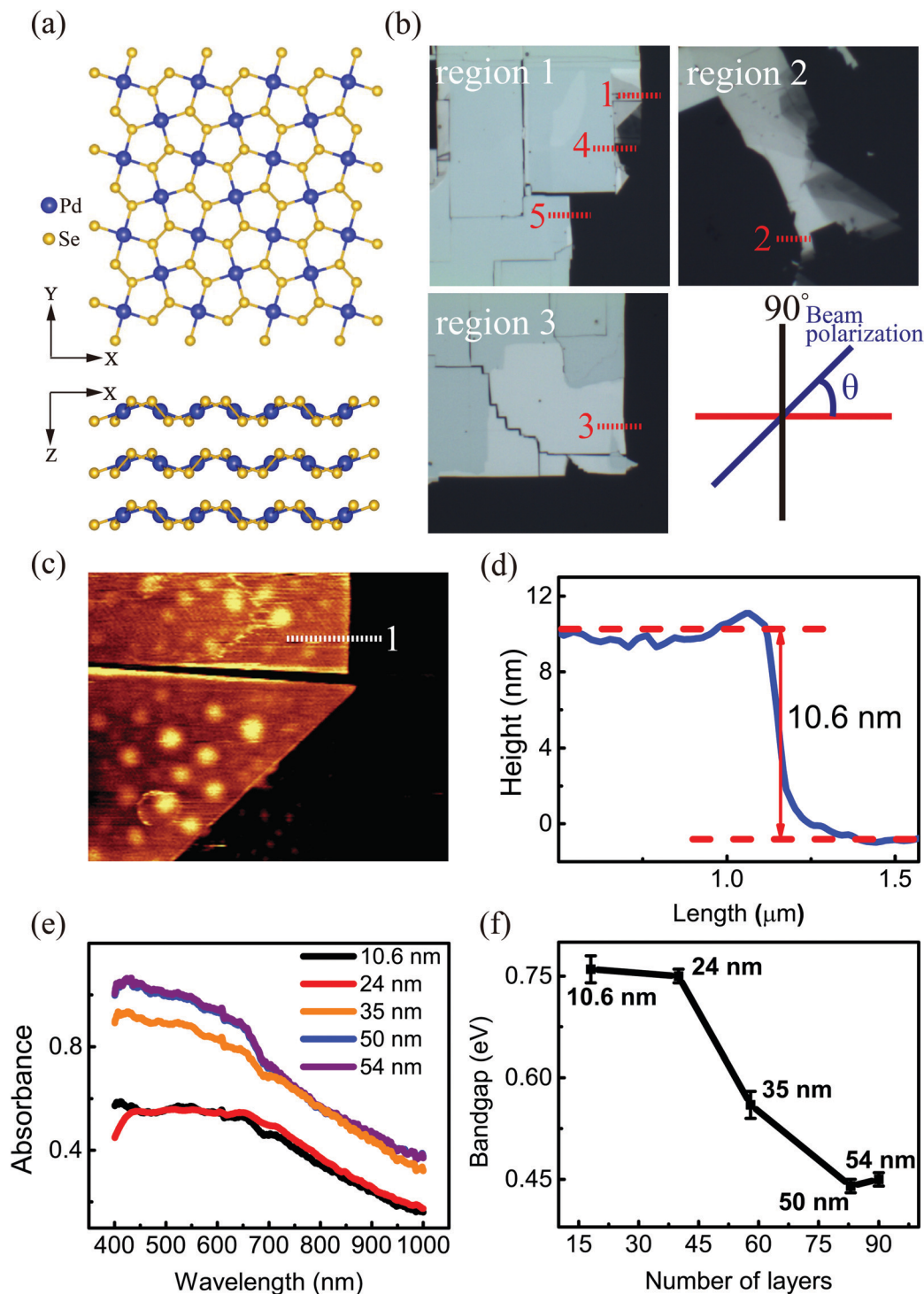
Fig. 1 Characterization of the PdSe 2 flakes. (a) Top and side views of the structure of the puckerd PdSe 2 crystal. (b) Optical microscope images of exfoliated few-layer PdSe 2 flakes on fused quartz, and the numbers 1–5 indicate the order of different thicknesses. All scale bars are 10 \mu m. (c) Corresponding atomic force microscope (AFM) image corresponding to number 1 in the first image of (b) labeled as region 1. The other two images in (b) are labeled as region 2 and region 3. (d) Corresponding thickness of PdSe 2 . (e) Absorption spectra of PdSe 2 flakes. (f) Thickness-dependent optical band gap extracted from the Tauc plots of \sqrt{\alpha h\nu} vs. h\nu for various numbers of PdSe 2 layers.
