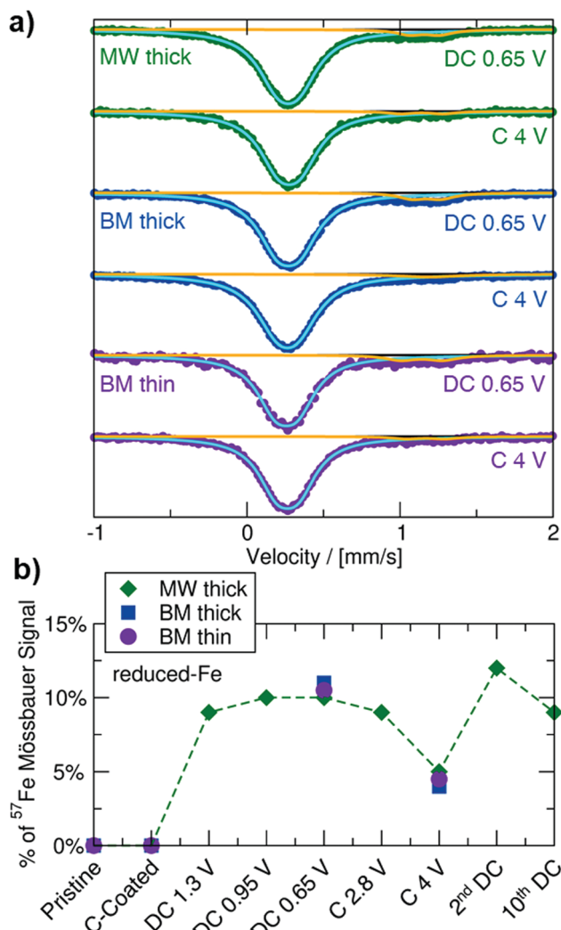
Fig. 4 ^{57}Fe Mössbauer of ex situ Na_3FeF_6 . (a) ^{57}Fe Mössbauer spectra of ex situ Na_3FeF_6 fit with two doublets for O_h - Fe^{3+} and reduced-Fe. (b) Change in the amount of ^{57}Fe signal ( \pm 2\% ) corresponding to the O_h - Fe^{3+} and reduced-Fe species at different states of charge.
