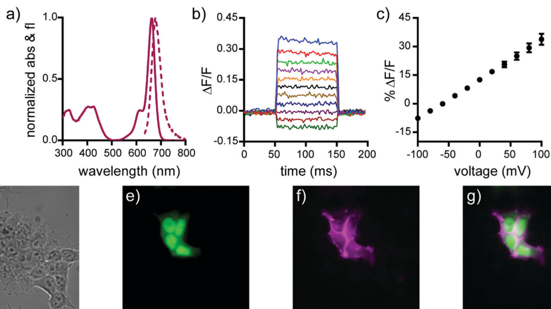
Fig. 1 Cellular and in vitro characterization of isoBeRST-Halo 7. (a) Normalized absorbance (solid line) and emission (dashed line) spectra of isoBeRST-Halo 7 in PBS, pH 7.4. (b) Plot of the fractional change in fluorescence of 7 vs. time for 100 ms hyper- and depolarizing steps ( \pm 100 mV in 20 mV increments) from a holding potential of -60 mV for single HEK cells under whole-cell voltage-clamp mode. (c) Plot of \% \Delta F/F vs. final membrane potential. Data are mean \pm S.D. for n = 6 cells. (d-g) Wide-field microscopy images of HEK cells transfected with CMV-HaloTag-pDisplay and stained with isoBeRST-Halo 7 (50 nM, 30 min). (d) DIC image of HEK cells. (e) Nuclear EGFP fluorescence indicates HaloTag expression. (f) isoBeRST-Halo fluorescence. (g) Merge of fluorescence from EGFP (green) and isoBeRST-Halo (magenta). Scale bar is 10 \mu\text{m} .
