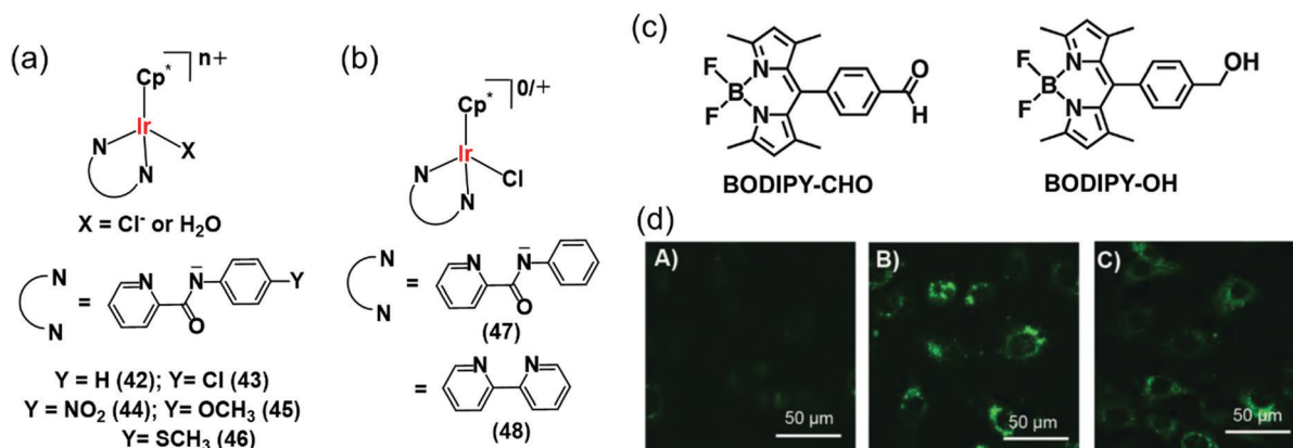
Fig. 14 (a) Ir III TH catalysts 42–46 which reduce aldehydes in PBS and cell culture media using NADH as hydride source. 29 (b) Organometallic Ir III catalysts 47 , 48 for intracellular conversion of aldehydes to alcohols. 30 (c) The fluorogenic BODIPY substrate (BODIPY-CHO) and its reduced form (BODIPY-OH). (d) Confocal microscope images of NIH-3T3 cells treated with (A) BODIPY-CHO (30 μM); (B) BODIPY-OH (30 μM) and (C) BODIPY-CHO (30 μM) + 47 (20 μM). Reproduced from ref. 30 with permission.
