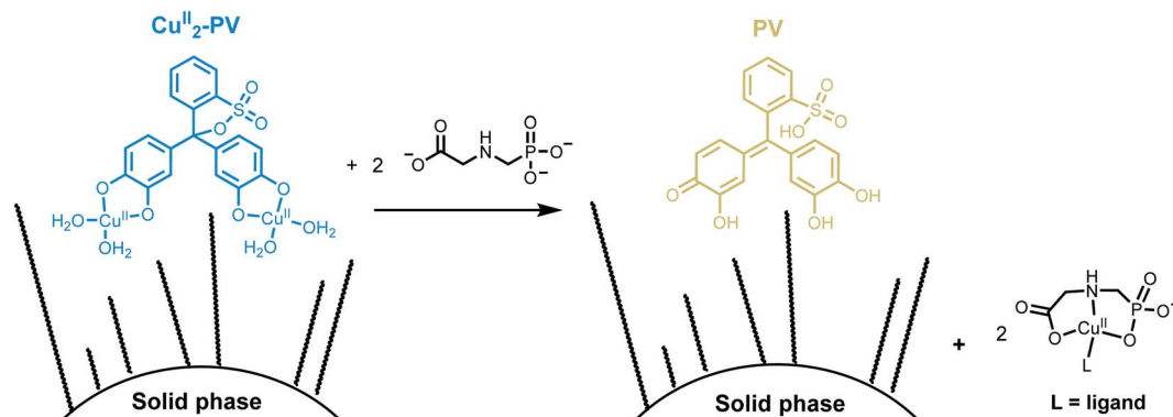
Fig. 2 Schematic representation of detection of GlyP with an immobilized \text{Cu}^{\text{II}}\text{-PV} complex by an indicator displacement assay using solid phase extraction.
