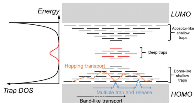
Fig. 2 (left) The trap DOS function represents shallow traps resulting from tail states (black) and deep traps (red) in the band gap. (right) Schematic spatial and energy diagram of an OSC containing localized trap states in the band gap. Tail states forming acceptor-like and donor-like shallow traps are shown in black, while deep traps are shown in red. Arrows represent different transport regimes possible in an OSC; band-like transport (black), MTR (blue) and thermally-activated hopping transport between localized states (orange).
