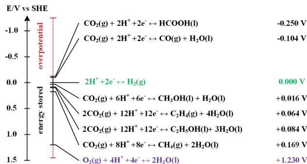
Fig. 2 Standard equilibrium potentials for hydrogen evolution half-cell reaction and several other half-cell reactions to reduce \text{CO}_2 into various products at 1 atm and 25^\circ\text{C} . Data presented was taken from Qiao et al. 27 (2014).
