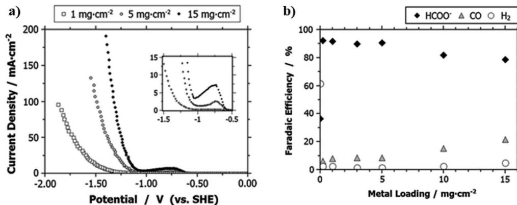
Fig. 12 (a) A comparison of CD for GDEs with various Sn loading as a function of potential. (b) The FE for HCOO - , CO and H 2 production for GDEs with different Sn loading at 50 mA cm -2 . All the experiment were conducted in the 0.1 M KHCO 3 aqueous electrolyte. Reprinted with permission from Kopljar et al. , 139 Copyright 2014, Springer Nature.
