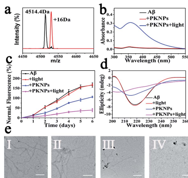
Fig. 3 (a) The mass spectra of A \beta 42 and A \beta 42 oxidized by PKNPs under laser excitation. (b) DNPH assay. (c) ThT fluorescence assay. (d) CD spectra of A \beta after various treatments. (e) TEM images of different A \beta samples: (I) A \beta , (II) A \beta + light, (III) A \beta + PKNPs, and (IV) A \beta + PKNPs + light. Scale bars are 200 nm.
