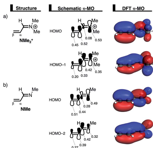
Fig. 6 Key occupied \pi -MOs (isovalue = 0.03 \text{ au}^{-3/2} ) computed at the equilibrium structures of (a) NMe 2 + and (b) NMe , where the MO-coefficients of the carbon and nitrogen 2p_z atomic orbitals, contributing to the occupied orbitals, are shown in the schematic \pi -MOs.
