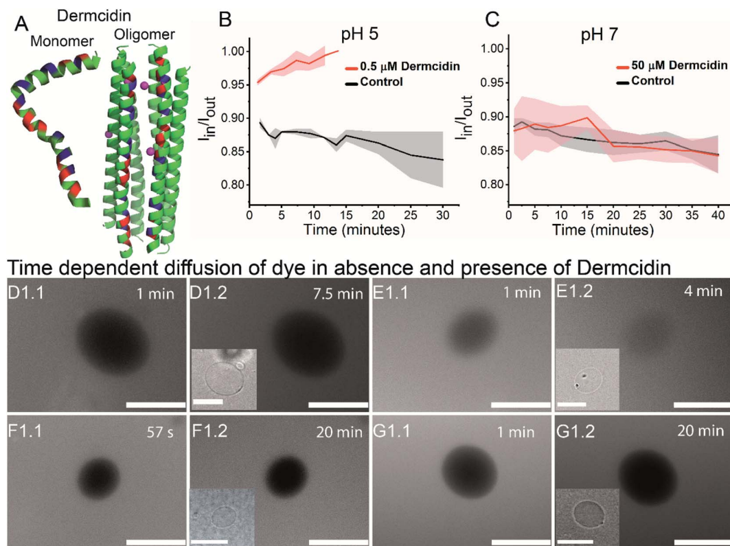
Fig. 5 Antimicrobial peptide permeability properties. (A) Dermcidin monomer and dermcidin oligomer stabilised by \text{Zn}^{2+} interacting with anti-parallel monomers made in the PyMOL Molecular Graphics System (the green colored residues are neutral, red colored are negatively charged and blue colored are positively charged residues at neutral pH and only two monomers are color coded in the oligomer for ease of viewing). Line graph depicting the I_{in}/I_{out} values with time (s) at (B) pH 5 and (C) pH 7. (D) Time-dependent uptake of Alexa Fluor 350 in the Gram-positive vesicle: without dermcidin at pH 5 (D1.1) at 1 minute, (D1.2) at 7.5 minutes, with dermcidin at pH 5 (E1.1) at 1 minute, and (E1.2) at 4 minute, without dermcidin at pH 7 (F1.1) at 57 seconds, (F1.2) at 20 minutes, and with dermcidin at pH 7 (G1.1) at 1 minute, and (G1.2) at 20 minutes. Scale bar 20 \mu\text{m} .
