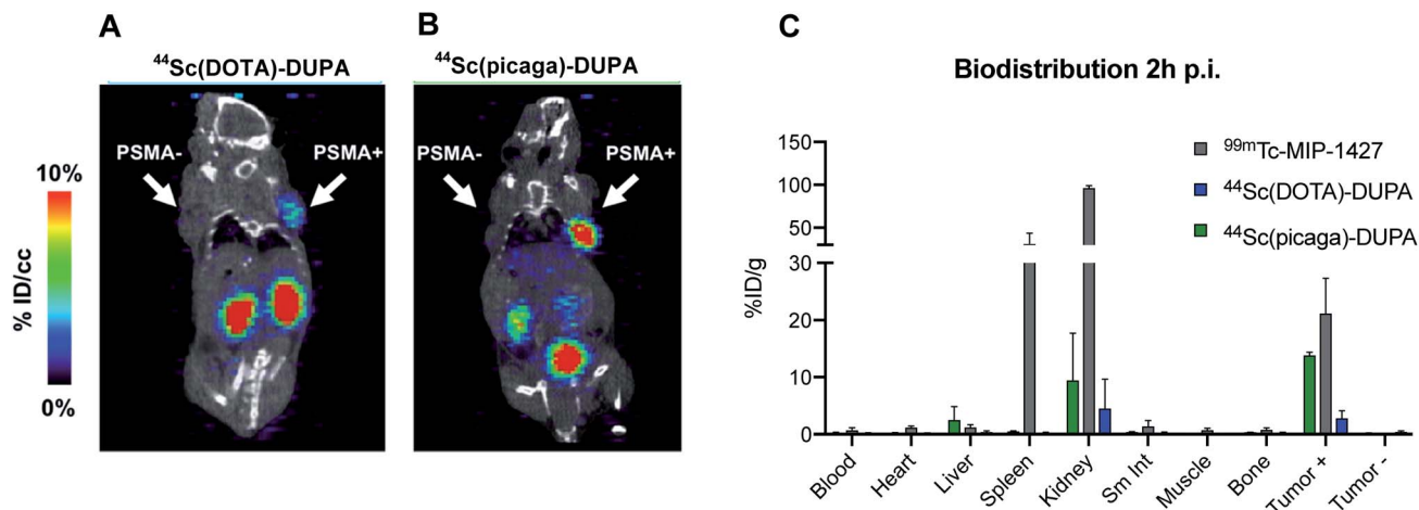
Fig. 7 Coronal PET-CT slices 90 min post injection show the superior tumor uptake achieved with ^{44}\text{Sc} (picaga)-DUPA (panel B) in comparison to ^{44}\text{Sc} -DOTA-DUPA (panel A), confirmed by the results obtained from the biodistribution analysis 120 min post injection (panel C).
