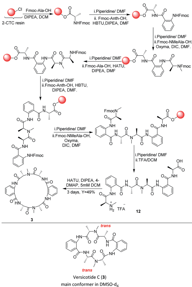
Scheme 4 SPPS and solution macrocyclization of versicotide C ( 3 )
