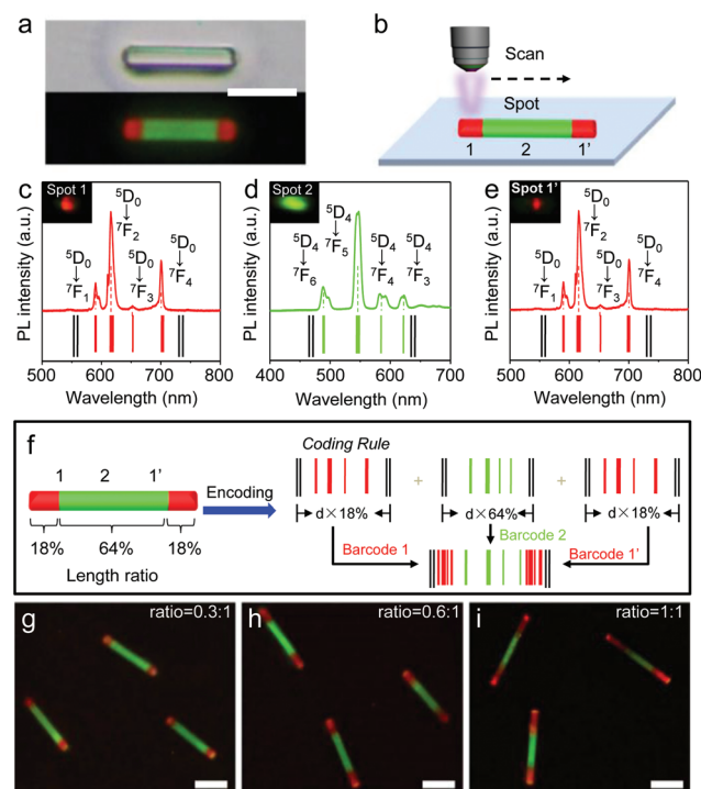
Fig. 8 (a) Bright-field and PL microscopy images of a segregated Ln-MOF heterostructure. Scale bar is 10 μm. (b) Schematic illustration of a heterostructure excited with a focused laser beam. Each part (marked as 1, 2, 1') of the heterostructure was selectively excited with a CW laser beam (375 nm). (c–e) Corresponding PL spectra collected from three different areas and the generated barcodes (marked as 1, 2, 1' shown in b). (f) Schematic illustration of the encoding strategy based on the segregated Ln-MOF heterostructure. According to the different block lengths in a heterostructure, the as-designed barcodes were compressed with the corresponding length ratio, which can be defined as the sub-barcode. The barcode was subsequently generated by combining the three parts of the sub-barcode. (g–i) PL images of the segmented structure with various block lengths. The block length can be precisely controlled by adjusting the epitaxy precursor-to-seed ratio in the reaction system. Scale bars are 10 μm. Reproduced with permission from ref. 42. Copyright 2019, Wiley-VCH.
