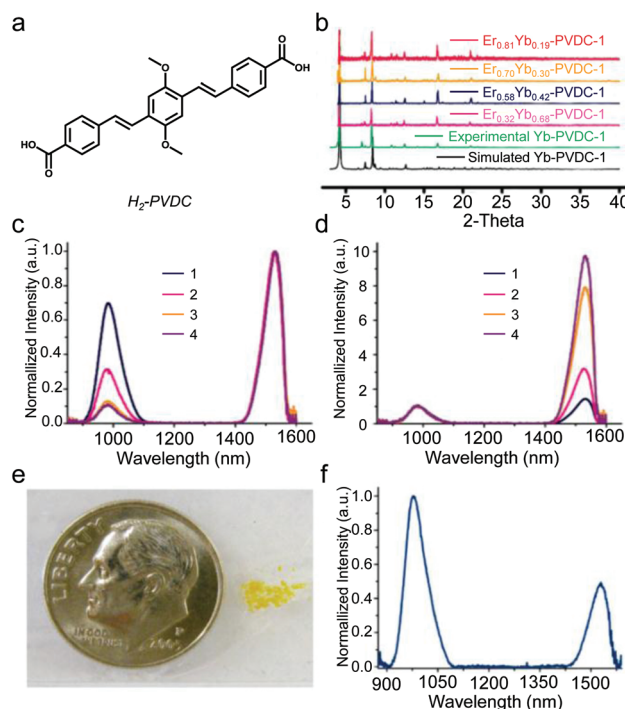
Fig. 9 (a) Molecular structure of the H 2 -PVDC, which was used to create polymetallic materials containing several different near-IR-emitting lanthanide cations. (b) Powder XRD patterns for Yb-PVDC-1 and other four luminescent metal-organic frameworks with varying lanthanide ion stoichiometries. (c and d) Yb 3+ (980 nm) and Er 3+ (1530 nm) emission spectra recorded upon 490 nm excitation: (c) normalized to the Er 3+ signal; (d) normalized to the Yb 3+ signal. With an increase in the amount of Er 3+ and a decrease in the amount of Yb 3+ , their respective emission intensities increase and decrease accordingly. (e) Anti-counterfeiting demonstration of the NIR barcoded materials. Sample of Er 0.70 Yb 0.30 -PVDC-1 needle crystals was dried and glued to a microscope slide (the dime is included for size perspective). (f) Corresponding PL spectrum of the sample shown in (e). Upon excitation at 490 nm, the Yb 3+ (980 nm) and Er 3+ (1530 nm) barcode was easily detected in the NIR range. Reproduced with permission from ref. 45. Copyright 2009, American Chemical Society.
