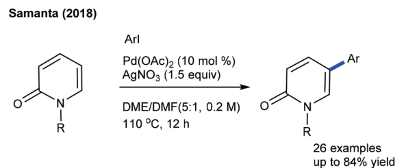
Scheme 9 C5-Arylation of pyridones.
