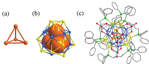
Fig. 22 (a) View of the \text{Ag}_4 inner core; (b) the structure of the two-shell \text{Ag}_4@ \text{Ag}_{24} ; and (c) total structure of \text{Ag}_{28}(\text{dppb})_6(\text{WO}_4)_4 . Adapted with permission from ref. 103. Copyright 2020, Royal Society of Chemistry.
