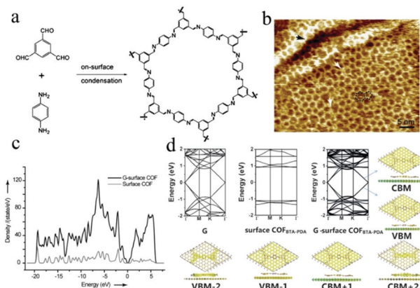
Fig. 13 (a) Reaction scheme of Schiff base condensation between benzene-1,3,5-tricarbaldehyde (BTA) and p -phenylenediamine (PDA) into hexagonal 2D surface COF BTA-PDA . (b) STM image of surface COF BTA-PDA on SLG-copper (single layer graphene grown by CVD on copper). A “5 + 7” defect is highlighted by an overlaid schematic model and two typical domain boundaries are marked by the white arrows. A perfect chain of hexagons crossing the step edge of copper is marked by a black arrow. (c) Density of states of G-surface COF BTA-PDA (the surface of COF BTA-PDA –graphene complex) and surface COF BTA-PDA (Fermi level is set at 0 eV). (d) The band structures of graphene, surface COF BTA-PDA , G-surface COF BTA-PDA and the decomposed charge density of G-surface COF BTA-PDA near the Fermi level (Fermi level is set at 0 eV). Copyright 2014, Angewandte Chemie International Edition. 46
