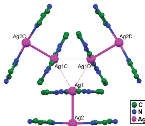
Fig. 1 The hexamer unit made of [\text{Ag}(\text{imid})_2]^{2+} cations in 1 , viewed along the crystallographic three-fold axis. There is a two-fold axis along each \text{Ag}^+ - \text{Ag}^+ vector, and hydrogen atoms are removed for clarity.
