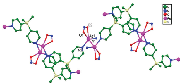
Fig. 20 The coordination environment around \text{Ag}^+ ions, with ligand-unsupported argentophilic interactions forming a zigzag chain in [\text{Ag}(\text{NO}_2)(\text{BPDMS})] , 31 .
