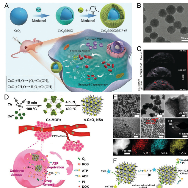
Fig. 4 Cobalt-/cerium-based nMOFs. (A) A schematic illustration, (B) TEM images and (C) PAI of \text{CaO}_2@DOX@ZIF-6 for combined chemo-/catalytic-therapy. Reproduced with permission. 36 Copyright: 2019, Wiley-VCH. (D) Mechanism of action, (E) characterization, and (F) oxidative-damage and reduced-energy-supply-enabled Ce-based nMOFs. Reproduced with permission. 37 Copyright: 2018, American Chemical Society.
