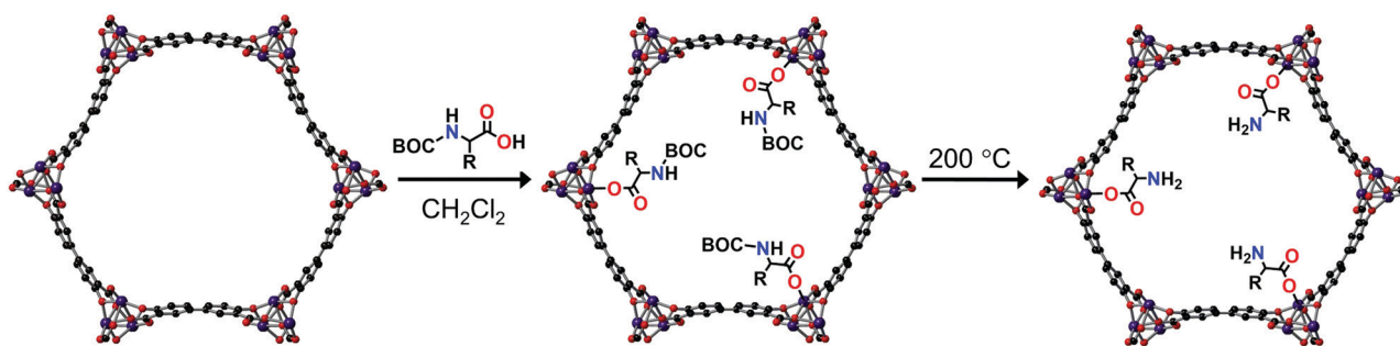
Fig. 1 Schematic of the appendage of BOC protected amino acids to the open \text{Mg}^{\text{II}} metal sites on S\text{-Mg}_2\text{dobpdc} to yield S\text{-Mg}_2\text{dobpdc}@(\text{BOC-Xxx}) (Xxx = Ala, Val, Pro) where R = \text{CH}_3 (alanine), ^i\text{Pr} (valine), \text{CH}_2\text{CH}_2\text{CH}_2 (proline) followed by the thermal deprotection of the BOC group to yield S\text{-Mg}_2\text{dobpdc}@(\text{Xxx}) (Xxx = Ala, Val, Pro). The appendage of amino acids to 50% of \text{Mg}^{\text{II}} metal sites is shown here for clarity. The atoms are represented as follows: magnesium (purple), carbon (black), oxygen (red).
