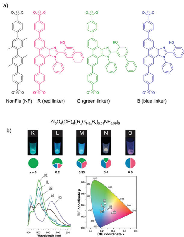
Fig. 4 (a) Solid solution formation with different RGB chromophore linkers in the UiO-type MOF [\text{Zr}_6\text{O}_4(\text{OH})_4(\text{NonFlu})_6]_x . (b) Luminescence images (top), spectra (bottom left) and CIE chromaticity coordinates (bottom right) (under \lambda_{\text{ex}} = 365 nm irradiation) of the one to three-component RGB MOFs (with chromophore composition indicated in the cake diagrams below the luminescence images). Reproduced from ref. 61 with permission from the American Chemical Society, copyright 2019.
