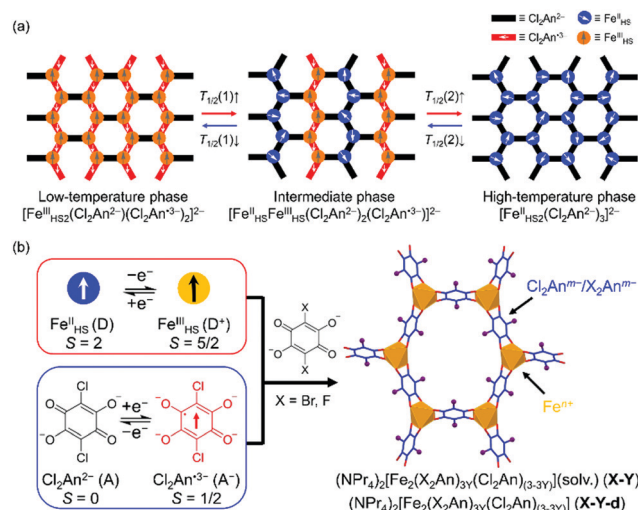
Scheme 1 Schematic representations of the investigated tetraoxolene-bridged Fe honeycomb layers. (a) The variations of charge-ordered states in 0 and 0-d , where for 0 , T 1/2(1) was T 1/2a (i.e., there was no high-temperature phase for 0 ), and for 0-d , T 1/2(1) and T 1/2(2) correspond to T 1/2b and T 1/2c , respectively. (b) Schematic route for the syntheses of site-doped solid solution compounds in this work.
