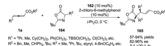
Scheme 51 Phosphine-catalyzed asymmetric additions of \gamma -substituted allenates and carbon electrophiles.
