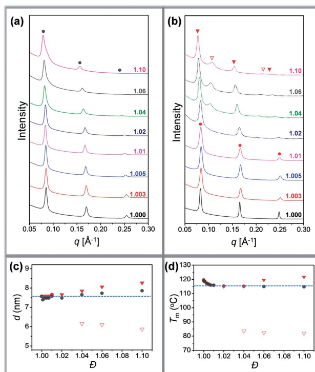
Fig. 3 (a and b) SAXS patterns of oLLA 22 series samples with varying \bar{D} crystallized at 60^\circ\text{C} (a) and 100^\circ\text{C} (b): solid line (region I); dashed line (region II). (c and d) Relationship between lamellar thickness and \bar{D} (c), and between melting temperature ( T_m ) and \bar{D} (d): solid circles (region I); triangles (region II). Only T_c = 60^\circ\text{C} (grey) and 100^\circ\text{C} (red) are shown for clarity. See Fig. S11† for more data.
