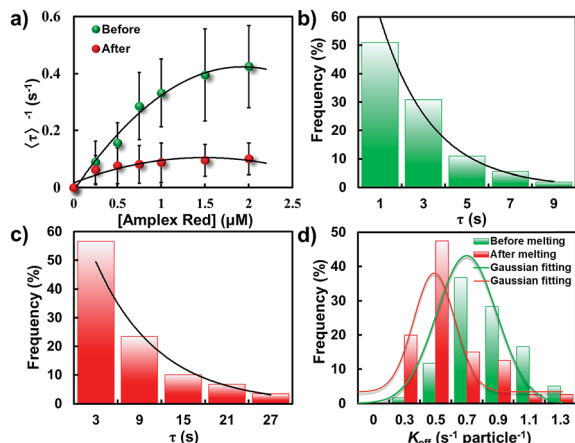
Fig. 6 Statistically analyzed catalytic activity of GNPs and GNRs. (a) Amplex red concentration dependence of \langle\tau\rangle^{-1} from gold nanoparticles before (green) and after (red) laser melting. Distributions of \tau from a single nanoparticle before (b) and after (c) laser melting, respectively. Solid lines are the exponential fits with a decay constant of k_{\text{eff}} = 0.84 and 0.69 s per particle for GNPs and GNRs, respectively. (d) Distributions of K_{\text{eff}} from individual gold nanostructures for the oxidative N -deacetylation reaction.
