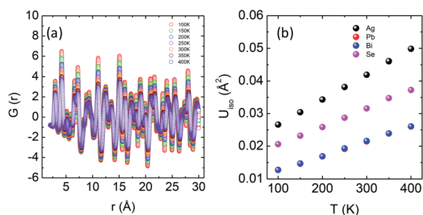
Fig. 5 (a) Temperature dependent atomic PDF G(r) plots of AgPbBiSe 3 plotted against real space. (b) Thermal ADPs of individual Ag, Pb, Bi and Se atoms plotted against temperature.
