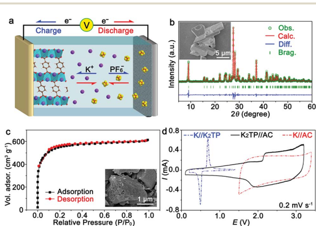
Fig. 1 (a) Schematic illustration of the KIHC with the configuration K_2TP//DME\text{-based electrolyte}/AC ; (b) XRD pattern, Rietveld-refined profile, and SEM image (inset) of K_2TP ; (c) nitrogen sorption isotherm and SEM image (inset) of AC; and (d) CV curves of half batteries and the KIHC.
