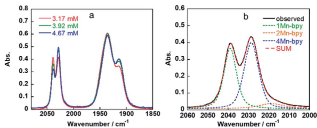
Fig. 5 IR spectra of fac - [\text{Mn}(\text{bpy})(\text{CO})_3(\text{MeCN})]^+ in DMF containing 1.3 M TEOA and different concentrations of \text{CO}_2 (a) and the curve-fitting result for the observed spectra at 3.17 mM \text{CO}_2 (b).
