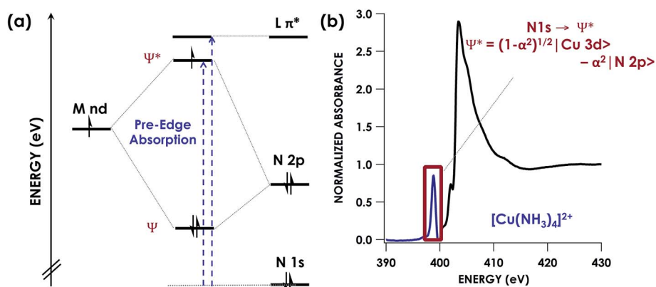
Fig. 1 (a) Simplified energy level diagram showing representative orbitals involved during pre-edge excitations in N K-edge XAS. (b) Representative N K-edge XAS spectrum of [Cu(NH 3 ) 4 ] 2+ with computationally validated pre-edge band assignment.
