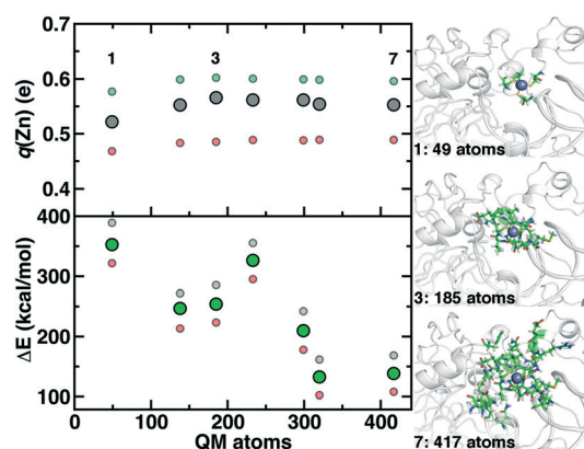
Fig. 11 Dependence of properties with QM region size: Zn Mulliken partial charge ( q(\text{Zn}) , in e ) shown at top left and rigid binding energy ( \Delta E , in kcal mol ^{-1} ) shown at bottom left. For each property, three snapshots are computed (40 ns in gray, 60 ns in red, and 100 ns in green), and the middle range symbol is shown in large solid symbols, whereas the upper and lower quantities are shown as translucent, smaller symbols. QM regions 1, 3, and 7 are shown at right in ball and stick representation.
