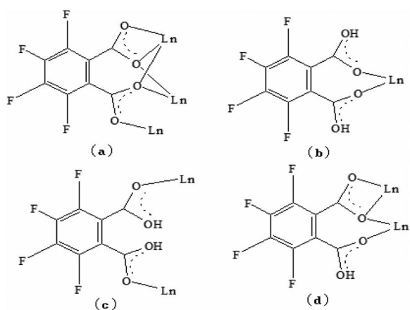
Scheme 1 Ligand models of Tfbda anion ligand in coordination polymers 1–6 .
