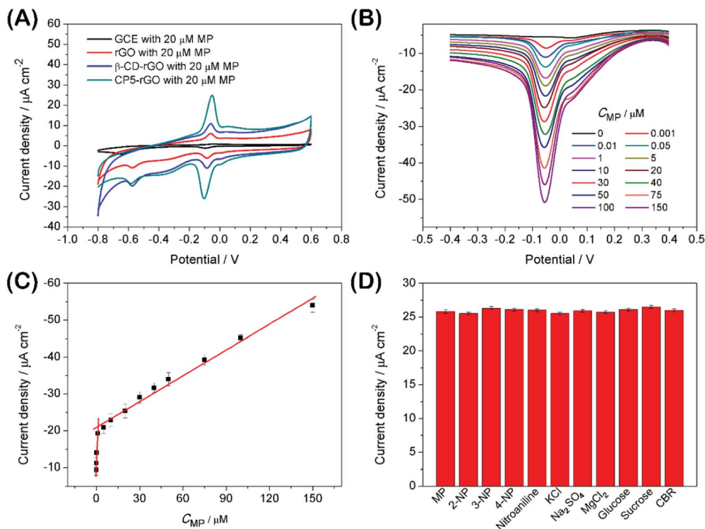
Fig. 4 The CV curves obtained for the redox reaction of 20 \mu M MP in PBS (0.1 M, pH 6.0) at bare GCE, rGO/GCE, \beta -CD-rGO/GCE and CP5-rGO/GCE (A). DPV curves obtained for the reduction of MP at CP5-rGO/GCE for different concentrations (B). Calibration plots of the reduction peak current at CP5-rGO/GCE versus concentration of MP under optimal conditions (C). Selectivity studies with different species in the developed MP detection strategy use DPV and keep all of the parameters constant. The MP concentration is 20 \mu M against the concentration of all of the other substances—this is held at 1.0 mM (D).
