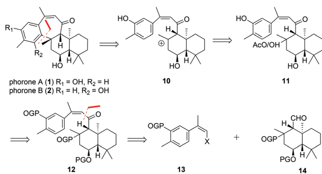
Scheme 2 Retrosynthetic analysis of phorones A (1) and B (2).
