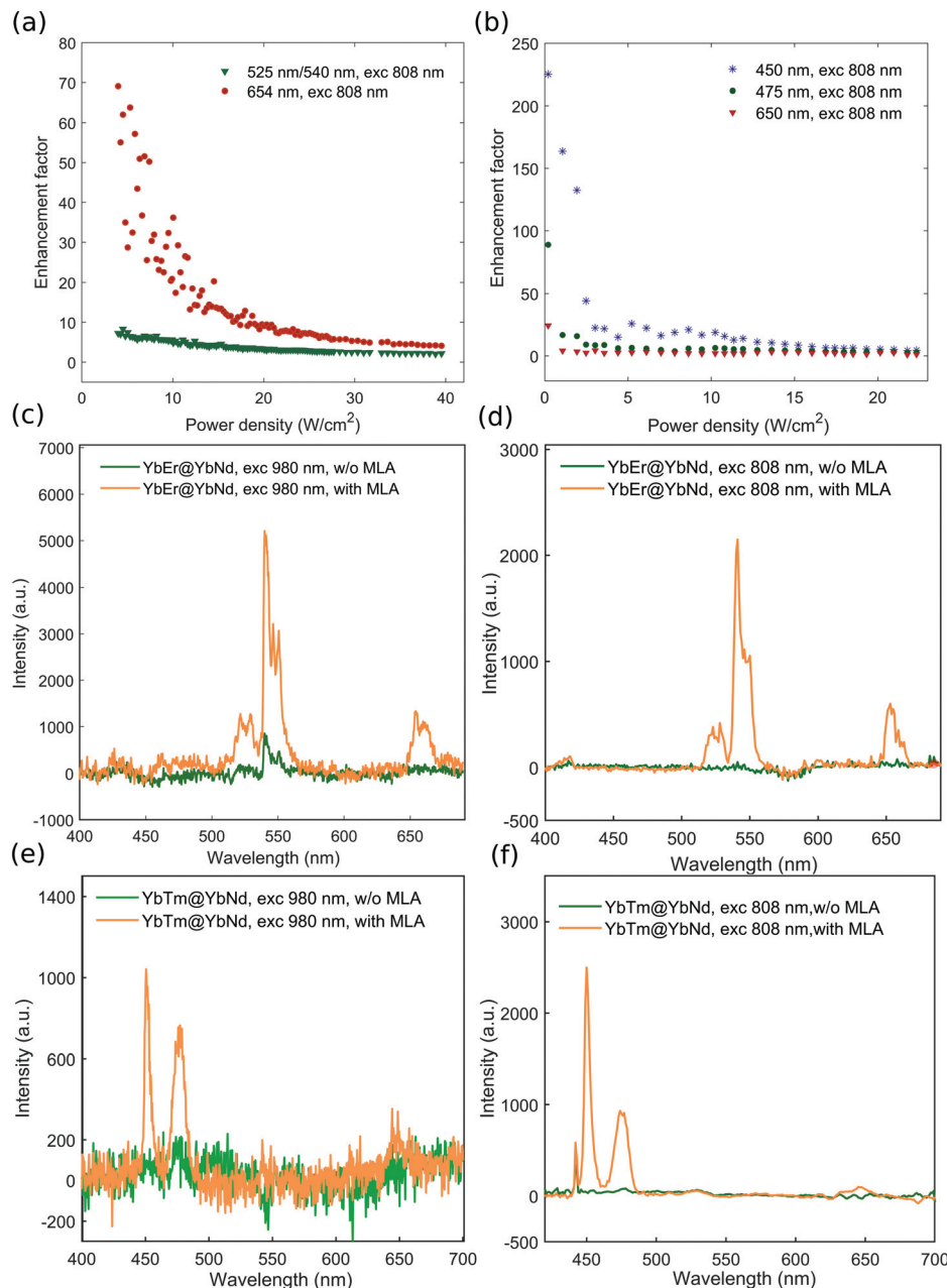
Fig. 3 Excitation intensity dependent enhancement factors induced by the addition of MLA of different emission bands of (a) \text{NaYF}_4\text{:}20\%\text{Yb}^{3+}, 2\%\text{Er}^{3+}@20\%\text{Yb}^{3+}, 30\%\text{Nd}^{3+} and (b) \text{NaYF}_4\text{:}20\%\text{Yb}^{3+}, 0.5\%\text{Tm}^{3+}@20\%\text{Yb}^{3+}, 30\%\text{Nd}^{3+} nanoparticles under 808 nm CW excitation. UCL spectra of \text{NaYF}_4\text{:}20\%\text{Yb}^{3+}, 2\%\text{Er}^{3+}@20\%\text{Yb}^{3+}, 30\%\text{Nd}^{3+} nanoparticles under (c) 980 nm and (d) 808 nm CW excitation with and without MLA light modulation (average excitation intensity: 0.1 \text{ W cm}^{-2} ). UCL spectra of \text{NaYF}_4\text{:}20\%\text{Yb}^{3+}, 0.5\%\text{Tm}^{3+}@20\%\text{Yb}^{3+}, 30\%\text{Nd}^{3+} nanoparticles under (e) 980 nm and (f) 808 nm CW excitation with and without MLA light modulation (average excitation intensity: 0.1 \text{ W cm}^{-2} ).
