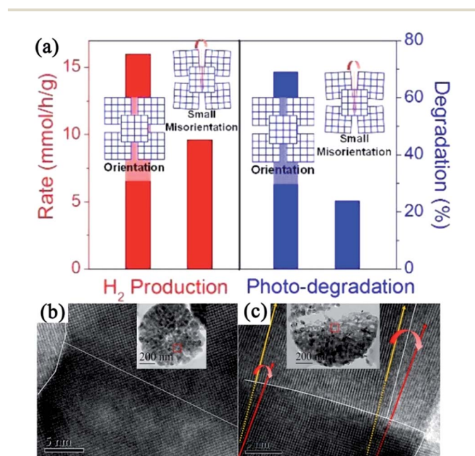
Fig. 4 (a) Schematic illustration of disordered and ordered aggregations of TiO 2 nanoparticles and their corresponding photocatalytic activities. (b) HRTEM image of TiO 2 mesocrystal with ordered orientation. (c) HRTEM image of TiO 2 mesocrystal with misorientation (crystal lattice mismatch). Adapted with permission from ref. 53. Copyright 2015 American Chemical Society.
