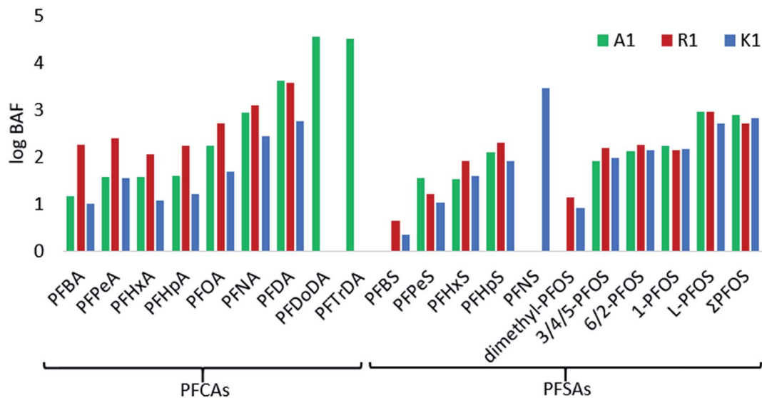
Fig. 4 The logarithmic bioaccumulation factor (BAF) on a wet weight basis ( \text{L kg}^{-1} ) of target PFCAs and PFSA (including four branched PFOS isomers, linear PFOS and \Sigma PFOS) for sites A1, R1 and K1. The BAFs could not be determined for some PFASs and sites due to values below MDL.
