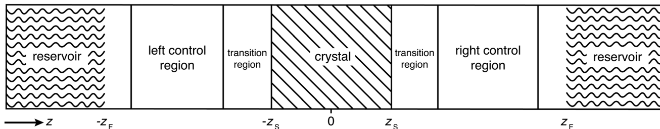
Fig. 1 Schematic of the C \mu MD method illustrating the segmentation of the simulation box. The two crystal surfaces are perpendicular to the z-axis and exposed to the solution at positions -z_S and z_S respectively. The external force positions are marked at -z_F and z_F .
