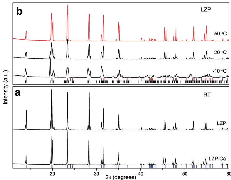
Fig. 1 (a) XRD patterns of L郑-1100 and L郑-Ca prepared by quenching; the markers (blue) are for the rhombohedral L郑 phase. (b) XRD patterns of L郑-1100 at selected temperatures; the top markers (red) are for the rhombohedral phase and the bottom markers (black) are for the triclinic phase.
