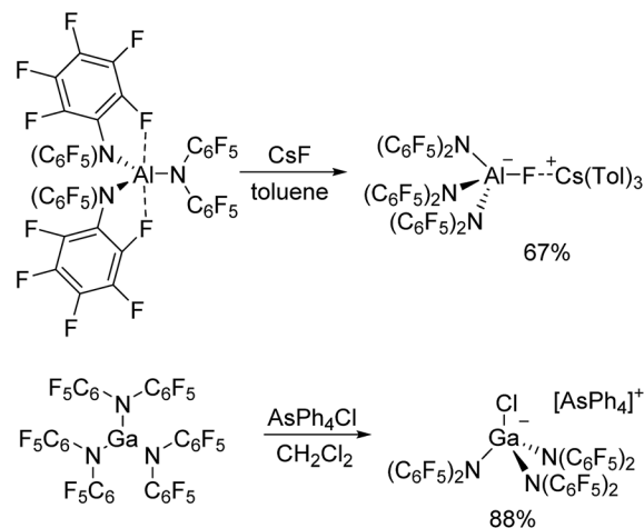
Scheme 4 Preparation of [\text{Cs(Tol)}_3]^+[\text{FAl(N(C}_6\text{F}_5)_2)_3]^- and [\text{AsPh}_4]^+[\text{ClGa(N(C}_6\text{F}_5)_2)_3]^- .
