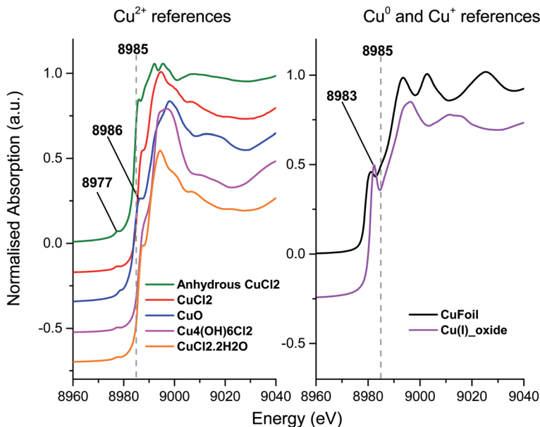
Fig. 2 Ex situ XANES spectra – Left: \text{Cu}^{2+} reference compounds, and right: \text{Cu}^0 and \text{Cu}^+ reference compounds, spectra are vertically offset for clarity.
