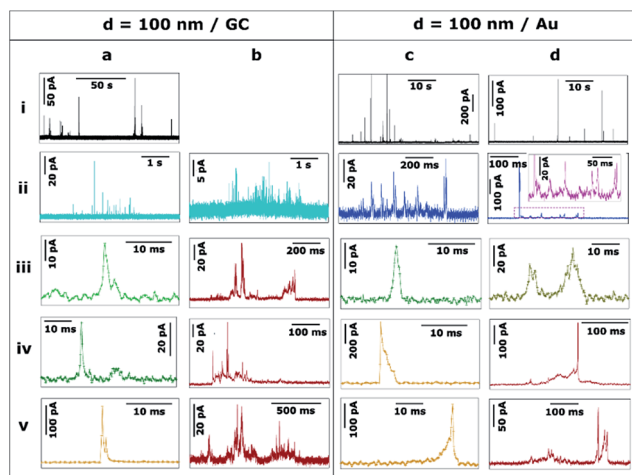
Fig. 5 Representative current transients obtained by applying E = +0.6 V vs. \text{Ag}/\text{AgCl} to a (a and b) GC and a (c and d) Au electrode with a solution containing Ag NPs with nominal diameter of 100 nm. The numbers i–v refer to different cases discussed in the text.
