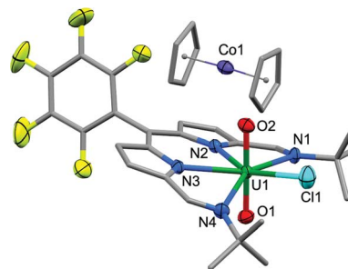
Fig. 7 Solid-state structure of the singly reduced [\text{CoCp}_2][\mathbf{2}] . For clarity, all hydrogen atoms, one THF solvent molecule, and a second molecule of [\text{CoCp}_2][\mathbf{2}] from the asymmetric unit are omitted (displacement ellipsoids drawn at 50% probability and fluorine atoms drawn in yellow). Selected distances/Å: U1–O1, 1.772(3); U1–O2, 1.779(3); U1–N1, 2.689(4); U1–N2, 2.482(3); U1–N3, 2.461(3); U1–N4, 2.670(4); U1–Cl1, 2.648(1). Selected angles/deg.: O1–U1–O2, 176.5(1); sum of equatorial bond angles around U, 364.9.
