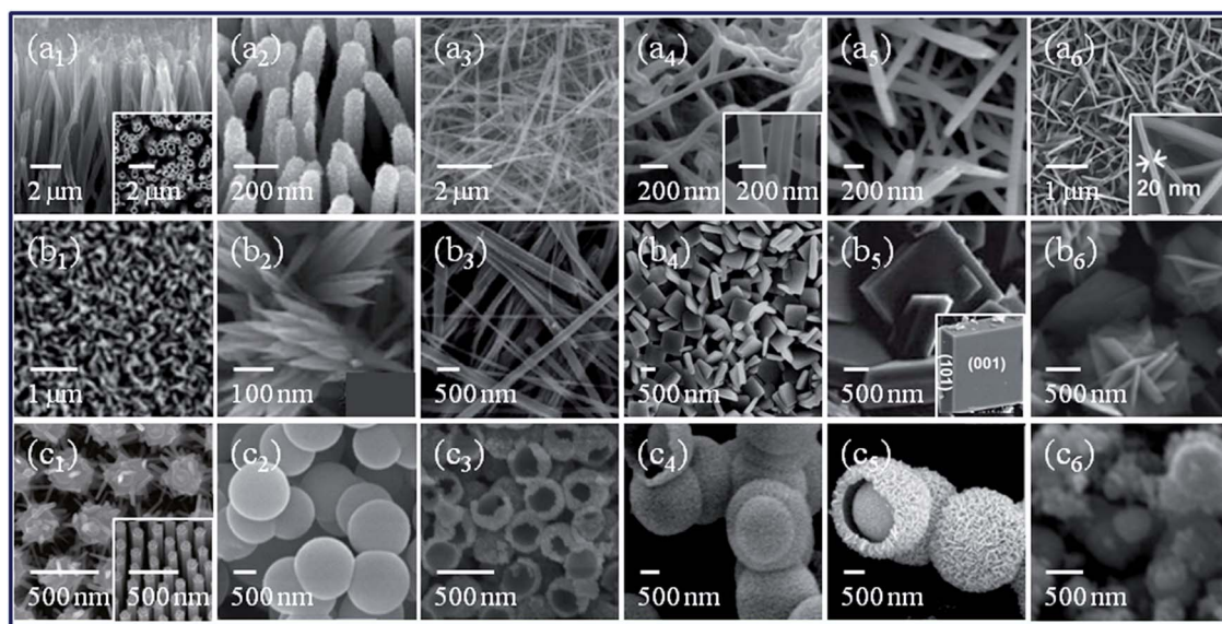
Fig. 11 SEM micrographs of anatase-TiO 2 nanostructures: (a 1 and a 2 ) nanotubes, (a 3 and a 4 ) nanofibres, (a 5 ) nanorods, (a 6 ) nanorods with nanoflakes, (b 1 ) nanorod arrays, (b 2 ) nanoribbons, (b 3 ) nanowires, (b 4 –b 6 ) nanosheets, (c 1 ) 3D network, (c 2 ) nanospheres, (c 3 ) nanospheres, (c 4 and c 5 ) nanospheres and (c 6 ) nanoparticles. Insets (a 1 , a 4 , a 6 , b 5 and c 1 ) provide the corresponding higher magnification images. Ref: [a 1 , a 2 ], 50 [a 3 ], 329 [a 4 ], 50 [a 5 ], 269 [a 6 ], 270 [b 1 ], 330 [b 2 ], 271 [b 3 ], 50 [b 4 ], 292 [b 5 ], 41 [b 6 ], 331 [c 1 ], 50 [c 2 ], 274 [c 3 ], 274 [c 4 , c 4 and c 5 ], 273 [c 6 ]. 275 (a 1 , a 2 , a 4 , b 3 and c 1 ) are reprinted with permission from ref. 50. Copyright 2014. American Chemical Society. (a 3 ) is reprinted with permission from ref. 329. Copyright 2005. Elsevier. (a 5 ) is reprinted with permission from ref. 269. Copyright 2013. The Royal Society of Chemistry. (a 6 ) is reprinted with permission from ref. 270. Copyright 2012. The Royal Society of Chemistry. (b 1 ) is reprinted with permission from ref. 330. Copyright 2004. The Royal Society of Chemistry. (b 2 ) is reprinted with permission from ref. 271. Copyright 2011. American Chemical Society. (b 4 ) is reprinted with permission from ref. 292. Copyright 2009. American Chemical Society. (b 5 ) is reprinted with permission from ref. 41. Copyright 2009. American Chemical Society. (b 6 ) is reprinted with permission from ref. 331. Copyright 2011. John Wiley and Sons. (c 2 , c 4 and c 5 ) are reprinted with permission from ref. 273. Copyright 2007. American Chemical Society. (c 3 ) is reprinted with permission from ref. 274. Copyright 2013. The Royal Society of Chemistry. (c 6 ) is reprinted with permission from ref. 275. VBRI Press.
