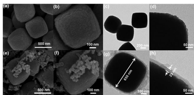
Fig. 1 SEM images (a and b) and TEM images (c and d) of \text{Fe}_2\text{O}_3 cubes, SEM images (e and f) and TEM images (g and h) of FC-23.
