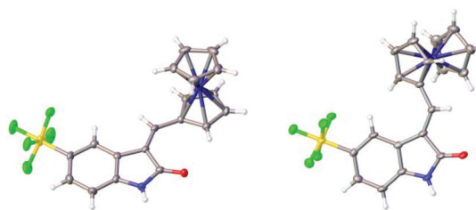
Fig. 4 Solid state structures of 12a and 12b.
