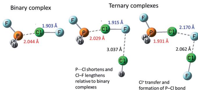
Fig. 4 Computational models of complexes H 2 FP...ClF, H 2 FP...ClF...ClH and H 2 FP...ClF...ClF, illustrating co-operativity in halogen bonding interactions. Adapted from DOI: 10.1039/c7fd00048k with permission from The Royal Society of Chemistry.
